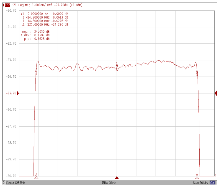
Ripple Variation Fo±14.80MHz
