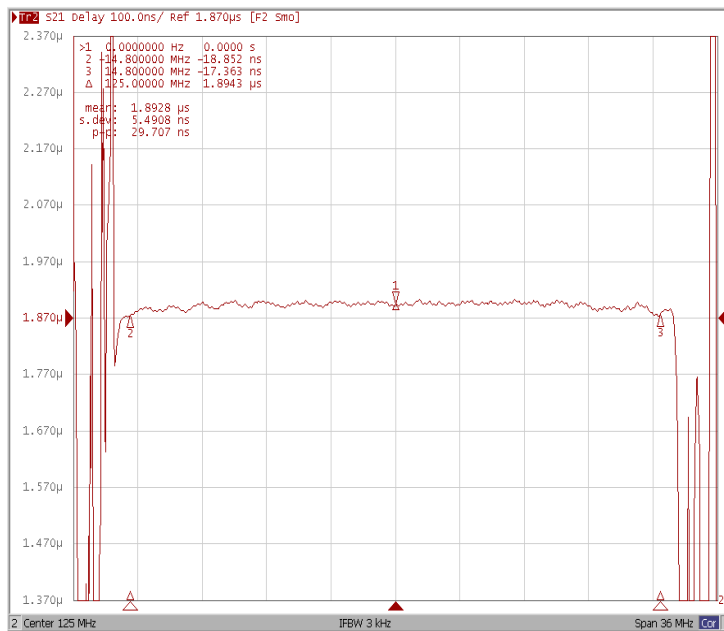
Group Delay Variation Fo±14.80MHz
